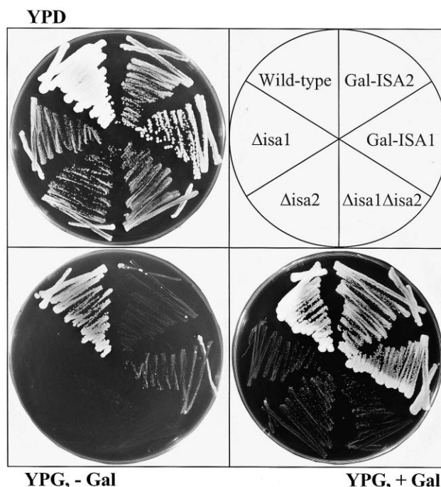
Fig. 1. Genetic inactivation of ISA2 impairs growth of yeast cells. Wild-type, \Delta isa1 , \Delta isa2 , \Delta isa1 \Delta isa2 , Gal-ISA1, and Gal-ISA2 cells were grown on rich media containing glucose (YPD), glycerol (YPG) or glycerol plus 0.2% galactose (Gal) for 3 days at 30°C.
